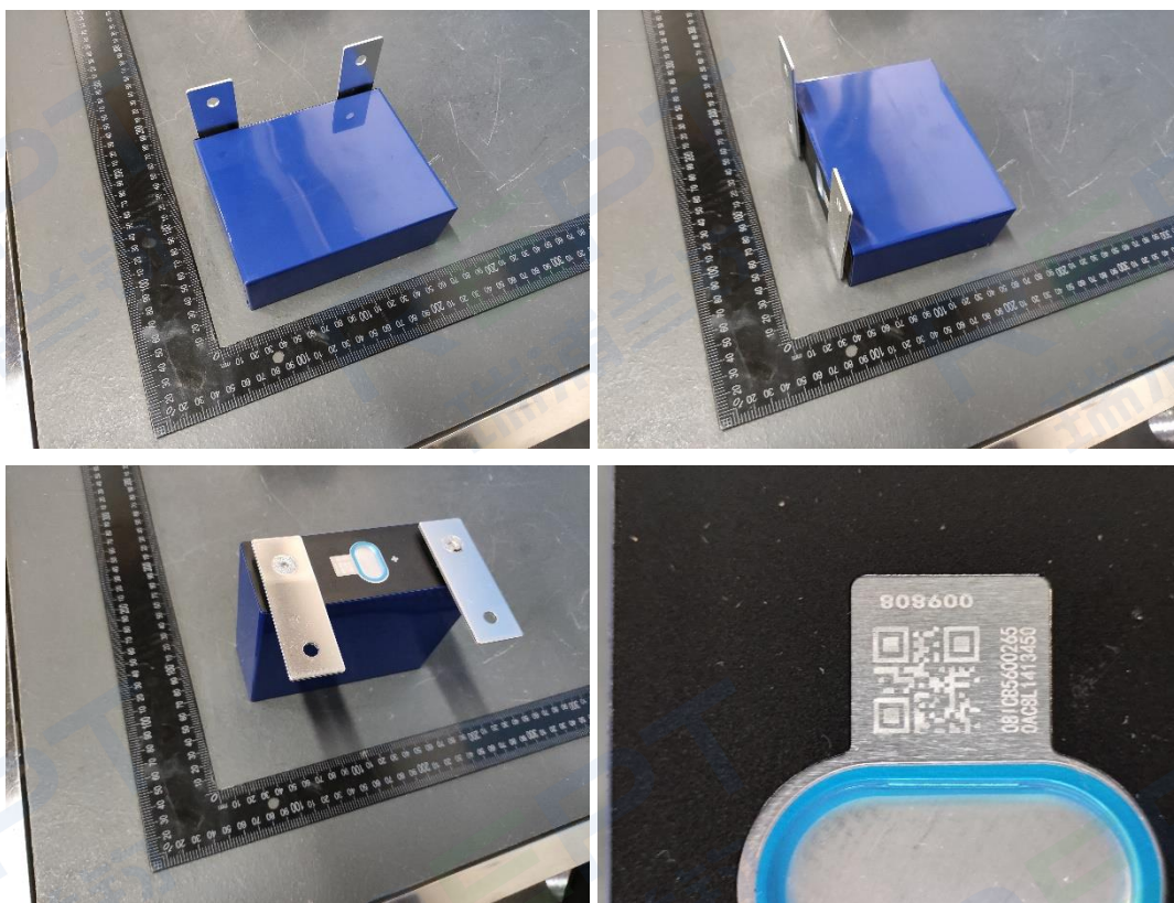
Cell/电芯 (CB56 3.2V 100Ah 320Wh)
