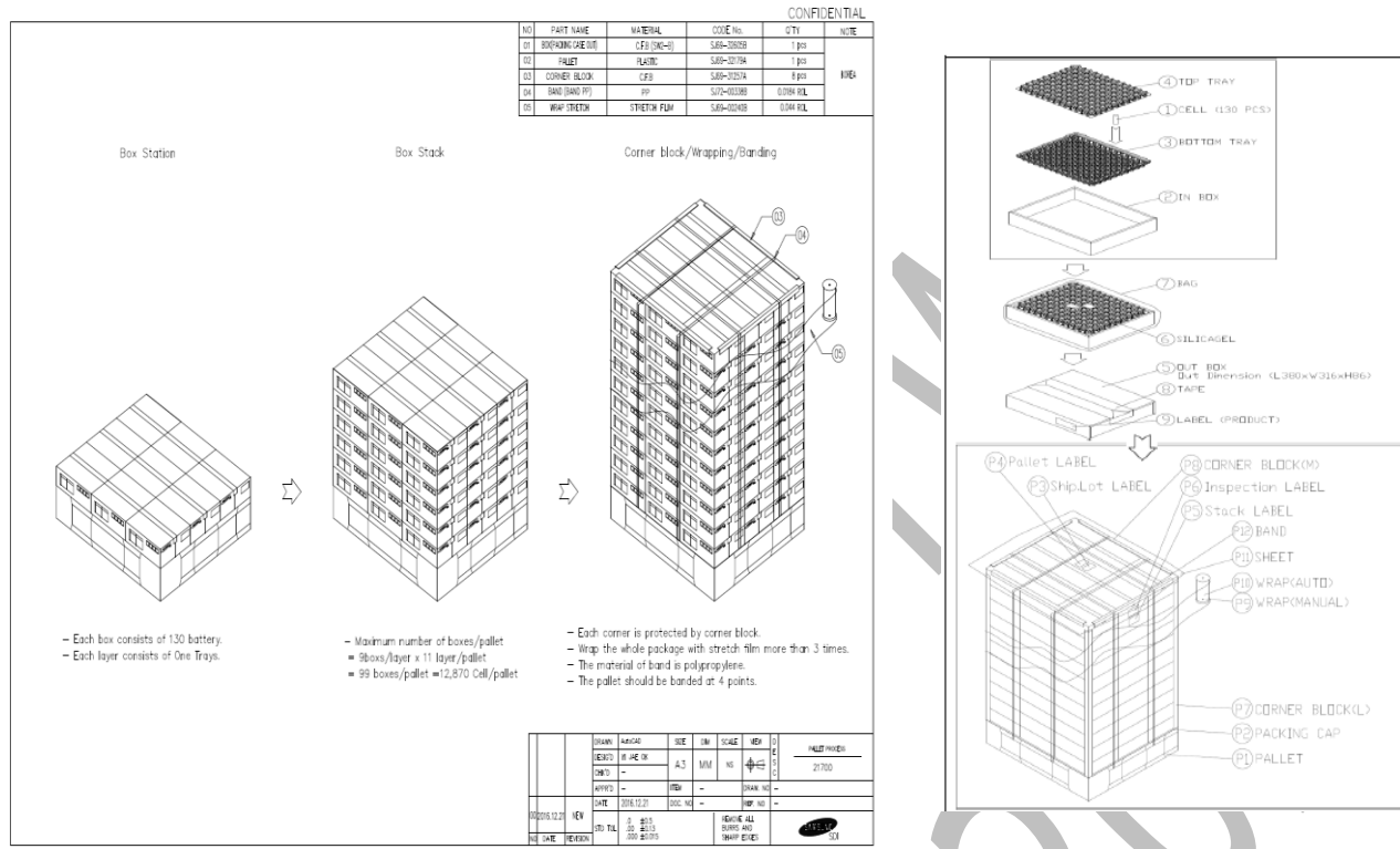
Fig. 2-5. Pallet packaging process
