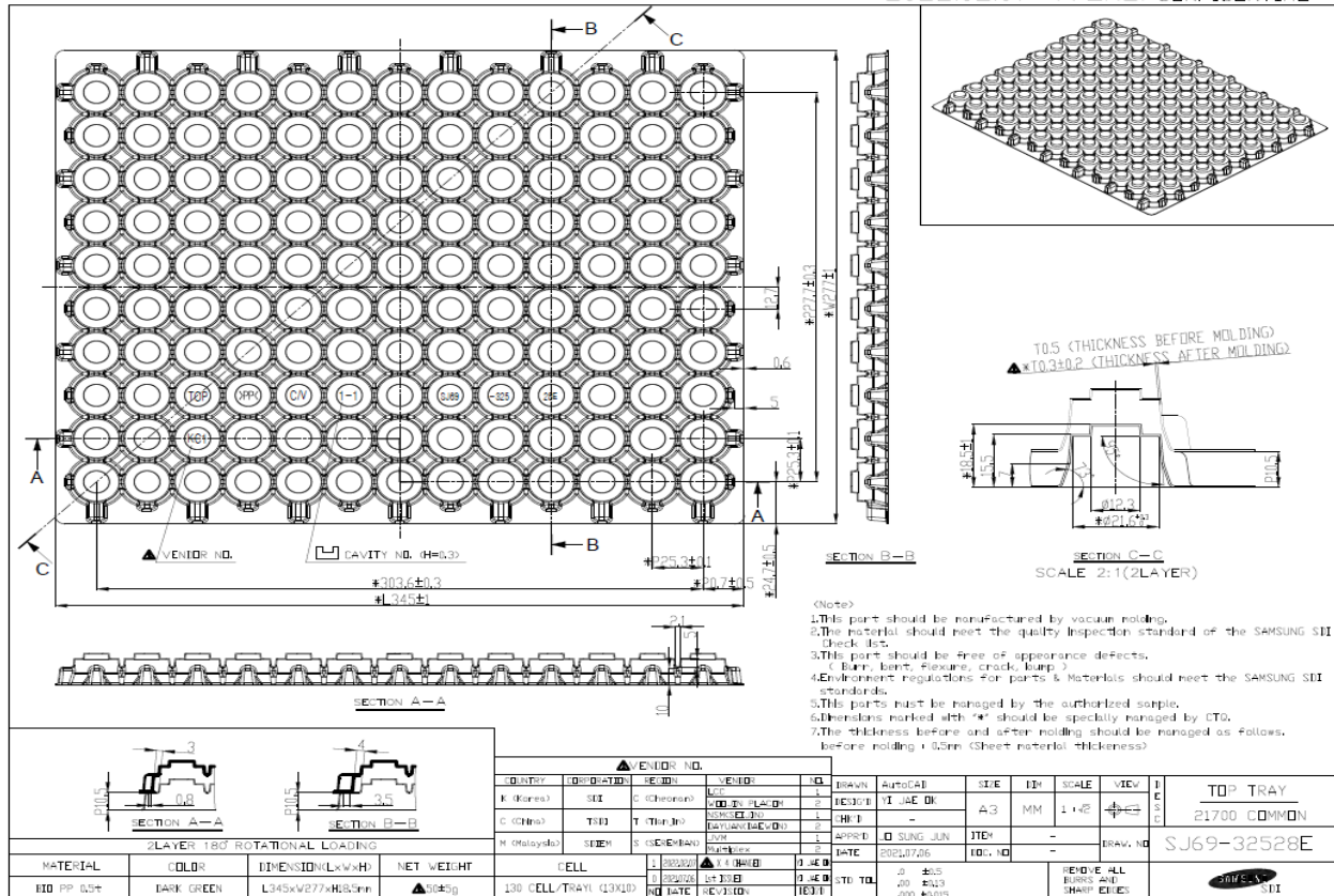
Fig. 2-3. Upper tray drawing.
